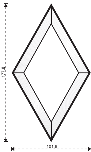
85384 47 4" x 7"
