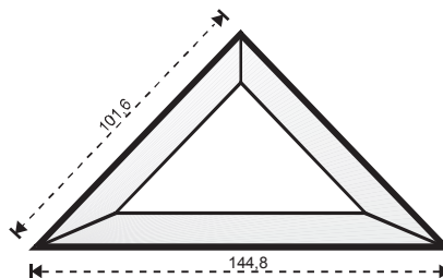
85380 57 4" x 4" x 5,7"
