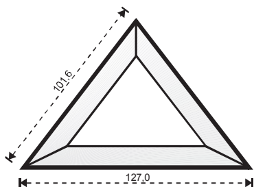
85380 45 4" x 4" x 5"
